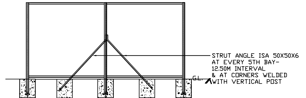
STRUT ANGLE DETAIL
